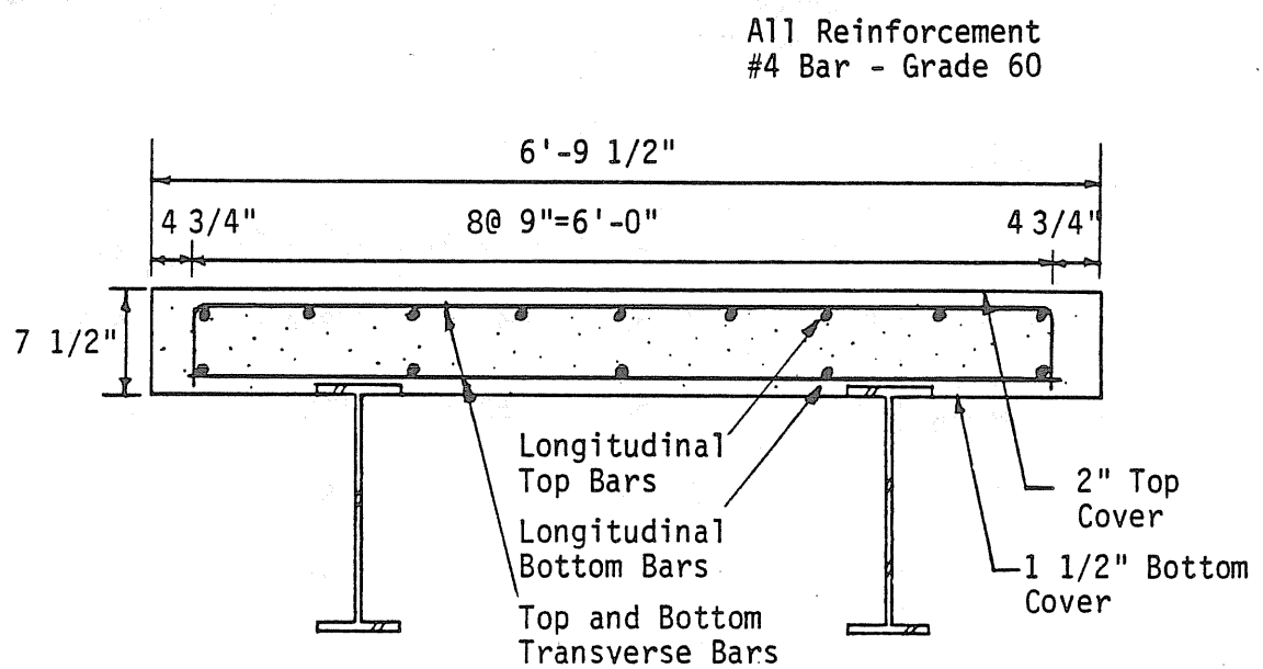
(b) Section A-A
