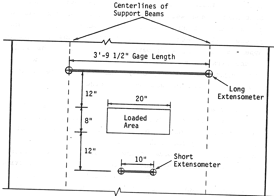
(a) Plan View of Instrumentation on Slab Surface
