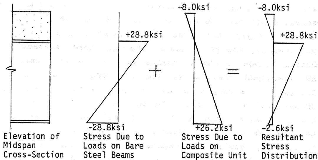
(b) Stresses on Second Unit Midspan Transformed Cross-Section
