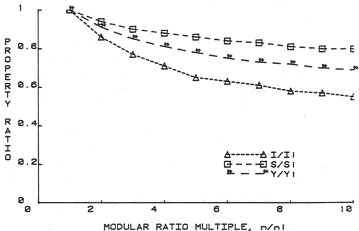
Figure K.4 Non-dimensionalized Section Properties vs. Modular Ratio Multiple
