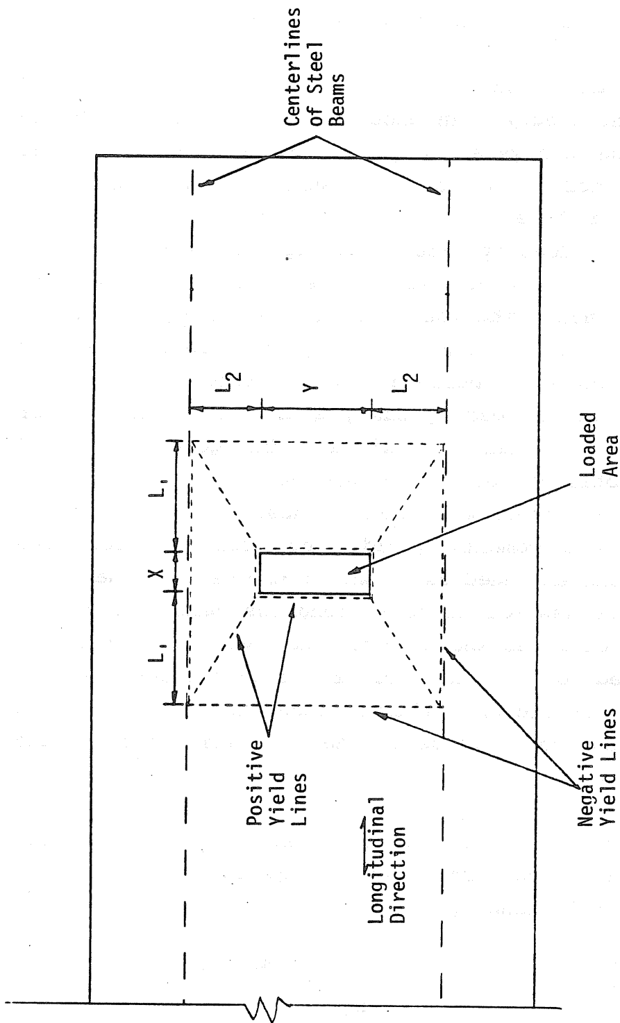
Figure 3.1 Yield Line Pattern for Bridge Unit Slabs
