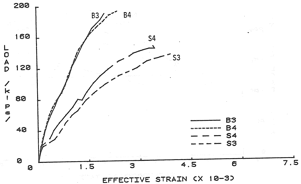
Figure I.5 Load vs. Effective Strain for Slabs with 0.57% Reinforcement Ratio, Phase XII Transverse Slab Strength Tests
