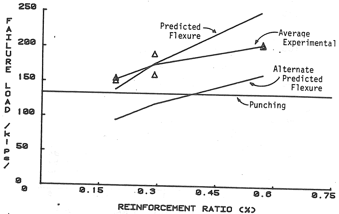
(a) First Bridge Unit Slabs
