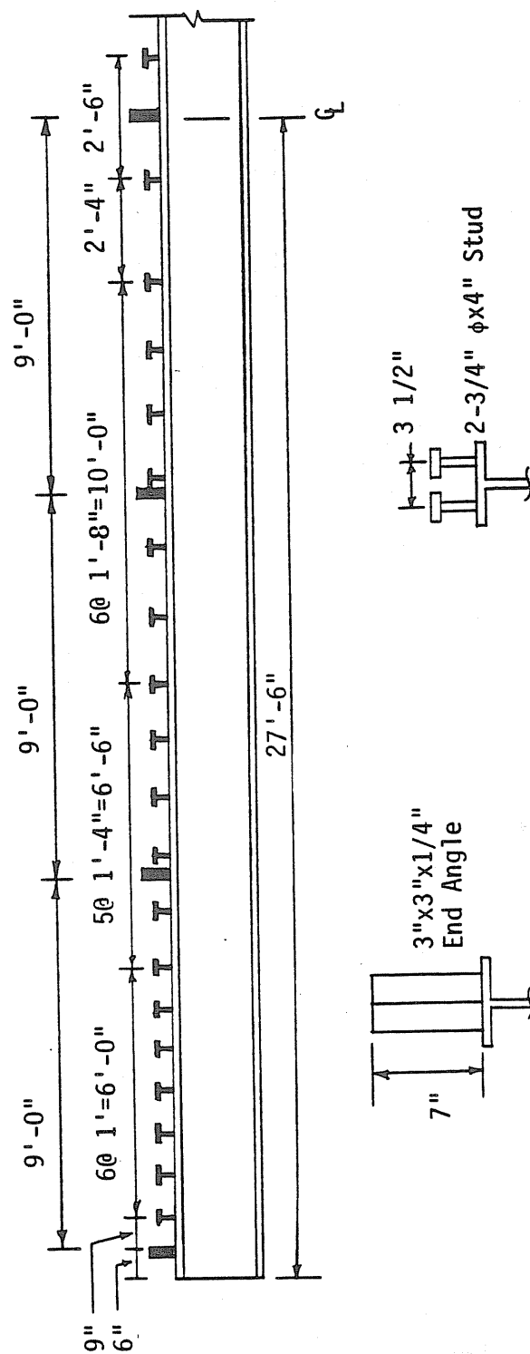
Figure B.3 Shear Connector Details Used for Second Bridge Unit
