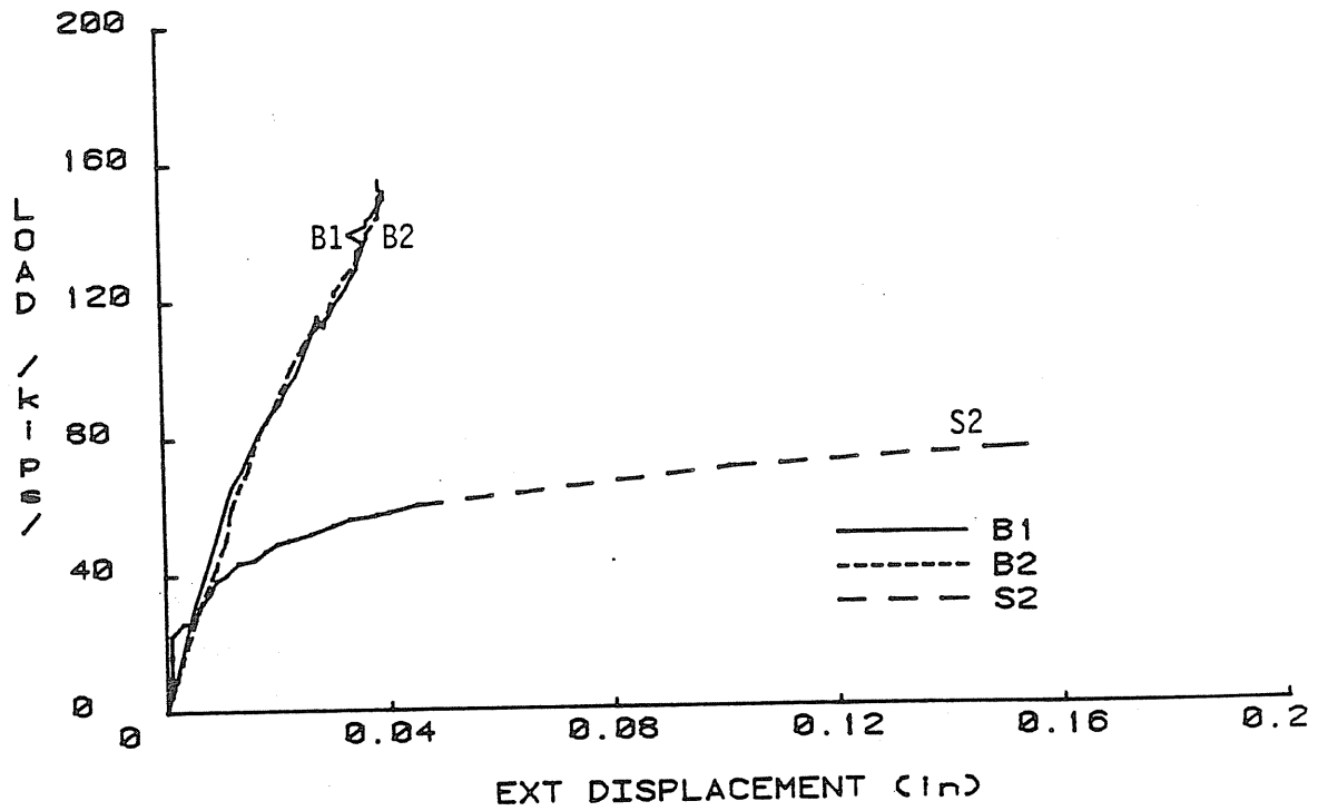
Figure I.2 Load vs. Restraint Displacement for Slabs with 0.19% Reinforcement Ratio, Phase XII Transverse Slab Strength Tests
