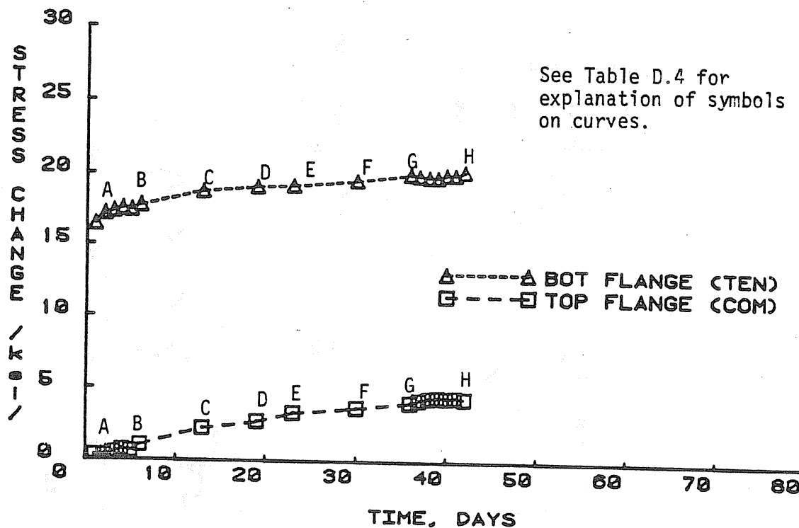
Figure D.15 Change in Stress in Beam Flanges vs. Time, Phase XI Sustained Loading Effects on Second Unit
