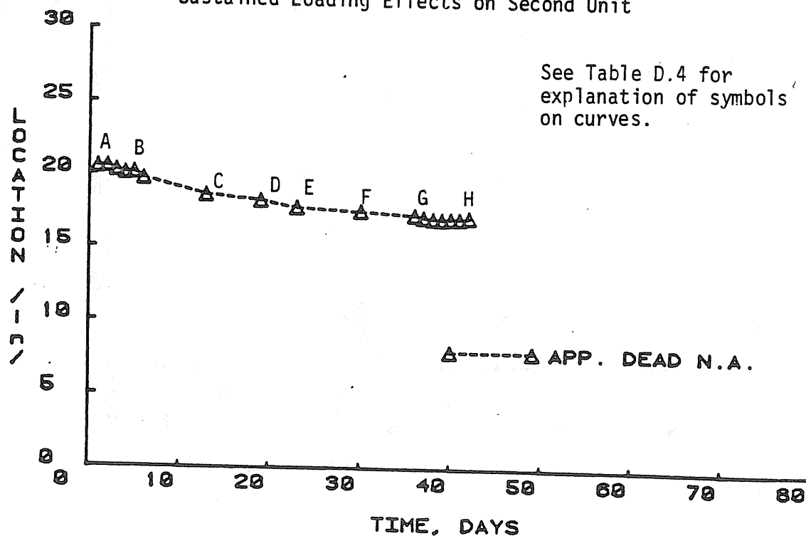
Figure D.16 Apparent Neutral Axis Location from Beam Bottom vs. Time, Phase XI Sustained Loading Effects on Second Unit
