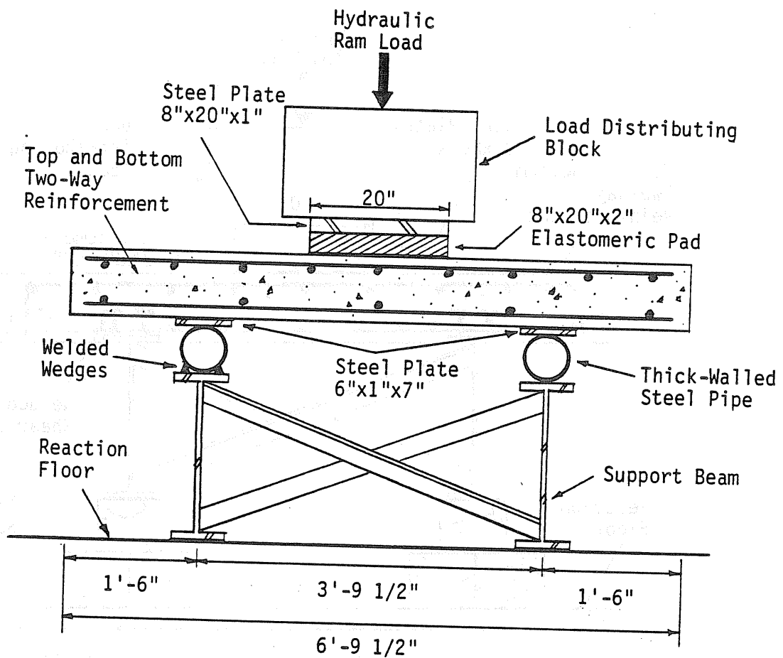
Figure C.11 Control Slab Transverse Slab Strength Test Setup
