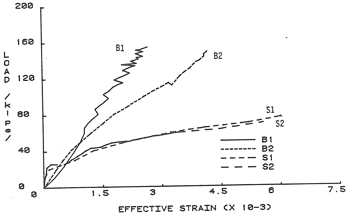
Figure I.1 Load vs. Effective Strain for Slabs with 0.19% Reinforcement Ratio, Phase XII Transverse Slab Strength Tests
