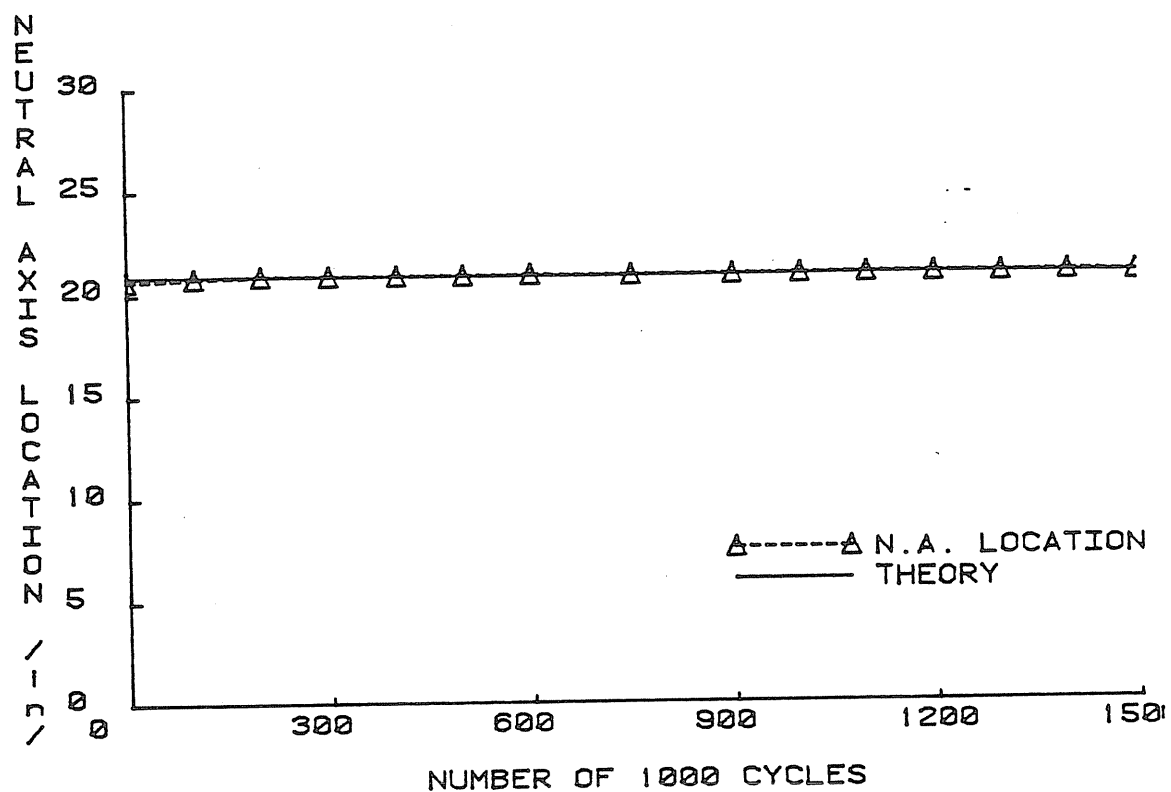
Figure E.11 Neutral Axis Location from Bottom of Beam vs. Number of Cycles, Phase V Repeated Loading
