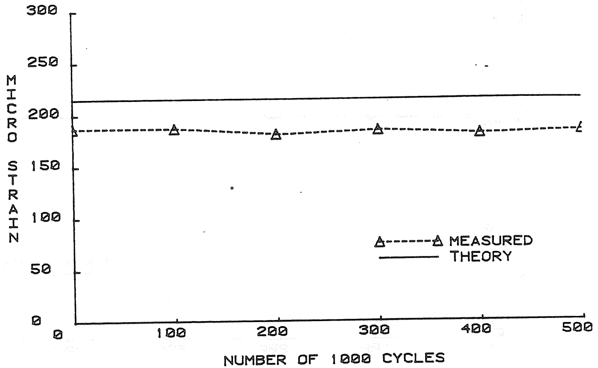
Figure E.24 Top of Concrete Strain vs. Number of Cycles, Phase IX Repeated Loading of Second Unit
