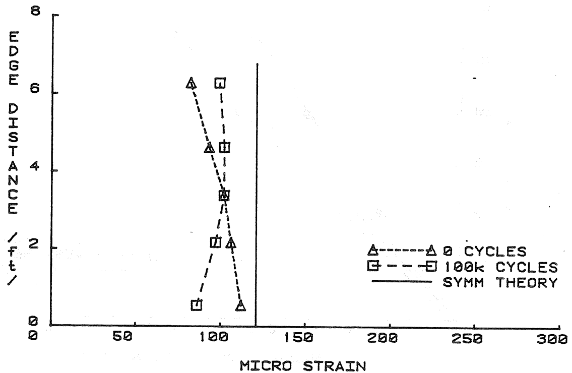
Figure E.18 Top Concrete Strain at Midspan Across the Slab Width, Phase VII Unbalanced Repeated Loading
