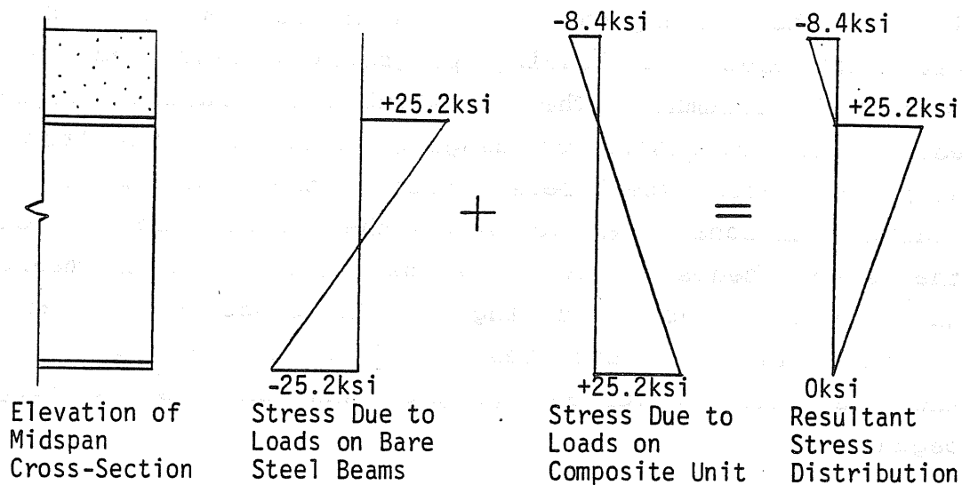
(a) Stresses on First Unit Midspan Transformed Cross-Section
