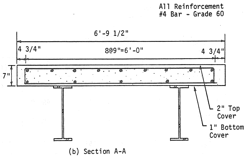
Figure B.4 Reinforcing Bar Details, Continued
