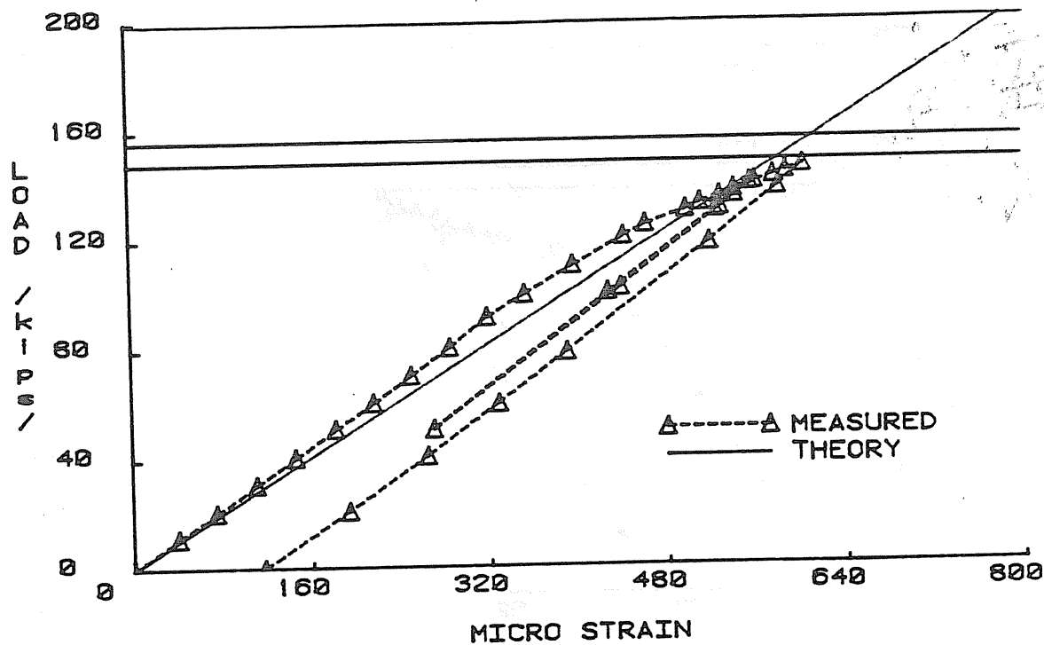
Figure F.11 Load vs. Strain of Concrete Surface, Phase X First Yield Failure Test of Second Unit
