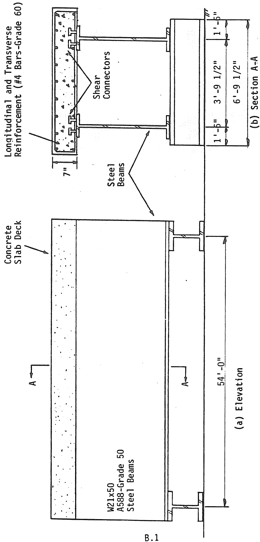
Figure B.1 Overall Dimensions of Second Bridge Unit
