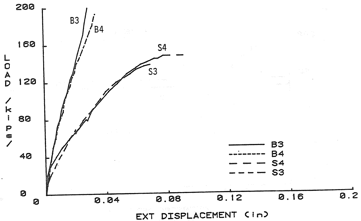
Figure I.6 Load vs. Restraint Displacement for Slabs with 0.57% Reinforcement Ratio, Phase XII Transverse Slab Strength Tests
