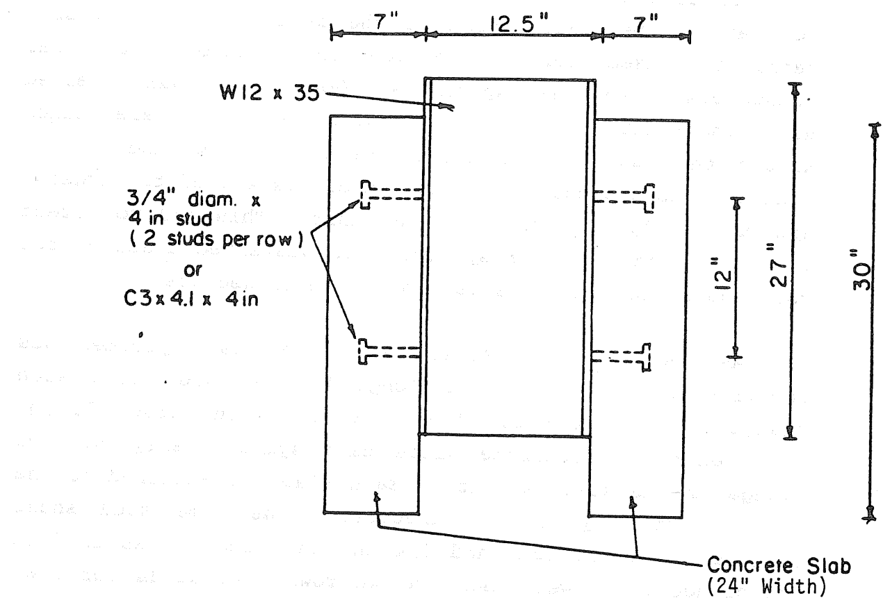
Figure H.1 Overall Dimensions of Shear Connector Specimens
