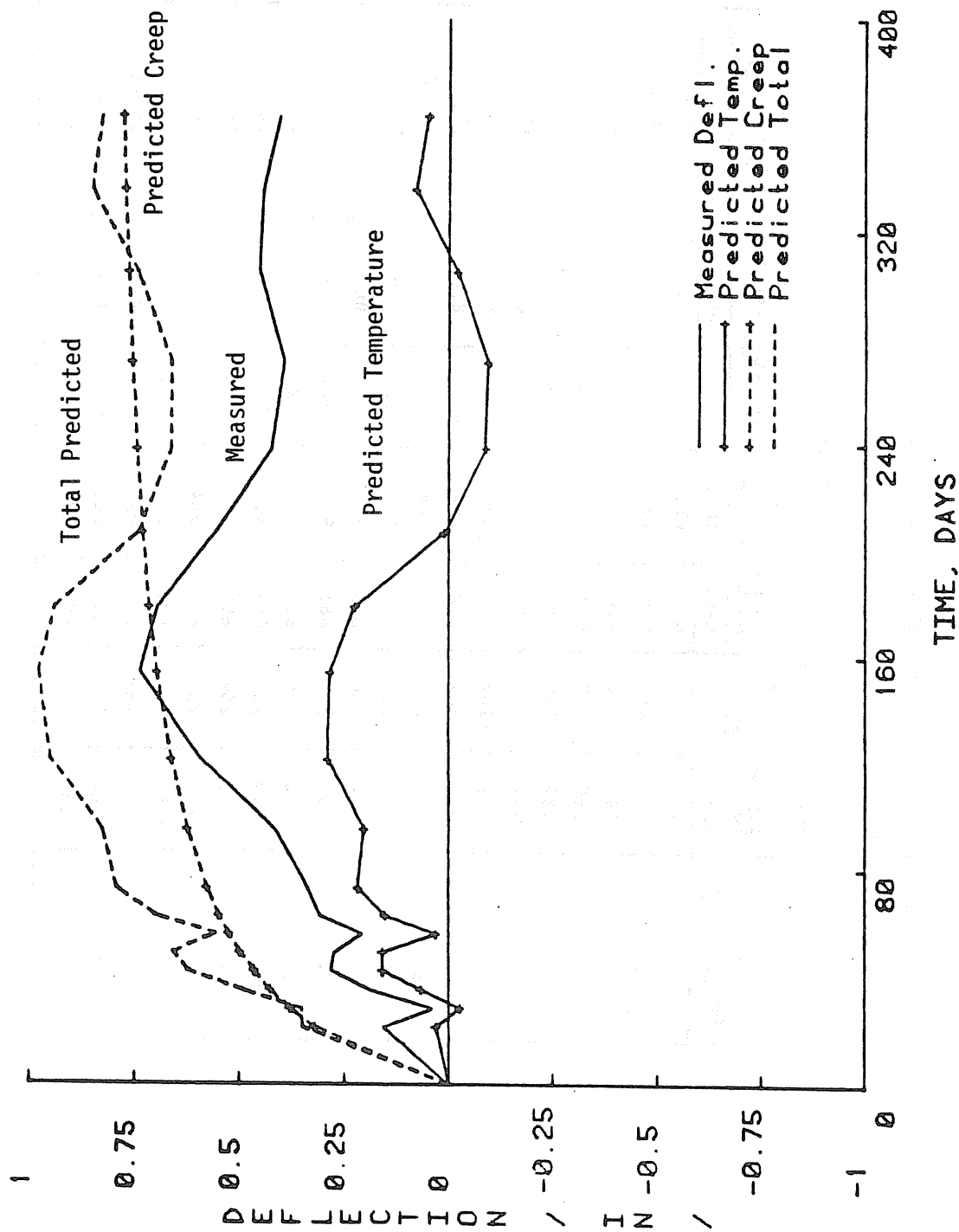
Figure D.2 Comparison of Measured Midspan Deflection Due to Shrinkage, Creep, and Temperature Effects with Predictions by Branson Method, Phase I Sustained Loading Test
