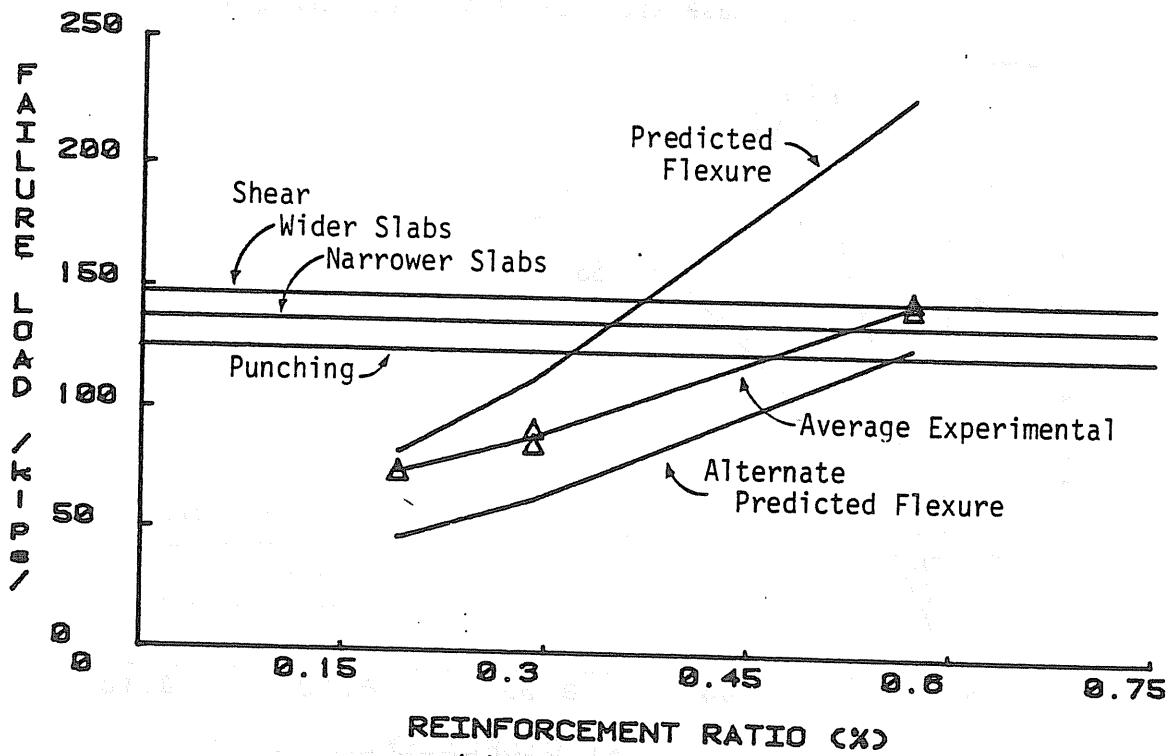
(b) Small Control Slabs
